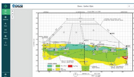
Live monitoring data displayed on dam cross-section
